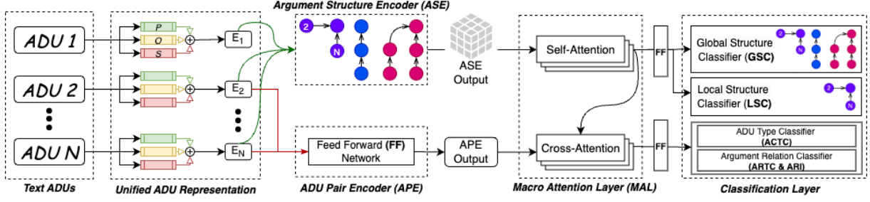
Figure 2: CU-MAM Architecture.
