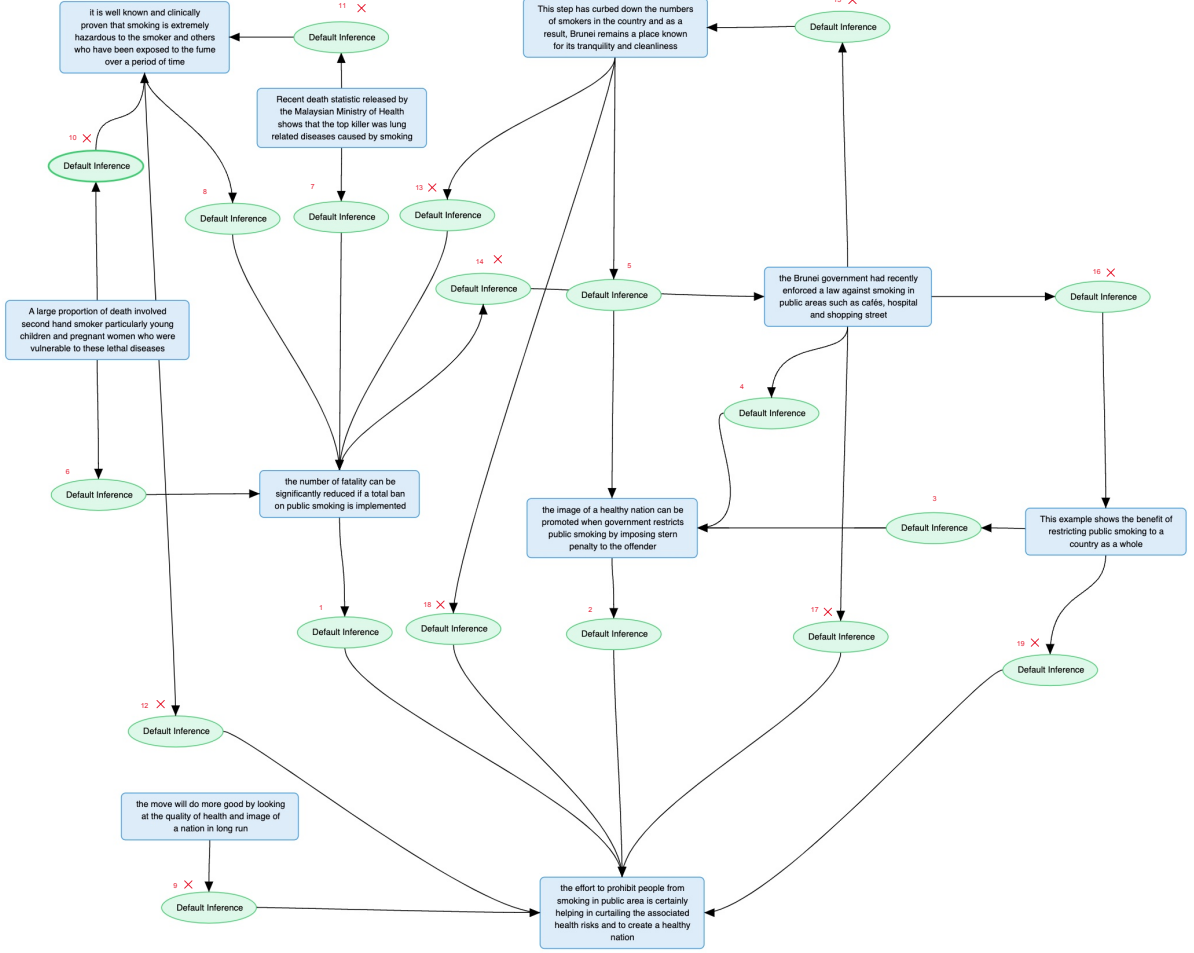
Figure 4: Example of error analysis. The argument map displays relations with arbitrary numbering, where incorrect predictions are marked with an (x) symbol.
